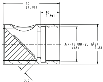
Right angle mirror
