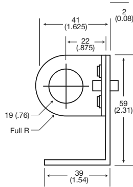
Adjustable Mounting Bracket
